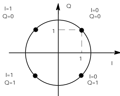
Figure 7: Bit mapping into QPSK constellation
