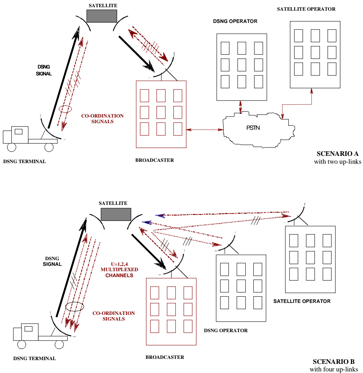
Figure 1: Example environments for DSNG and co-ordination transmissions by satellite
